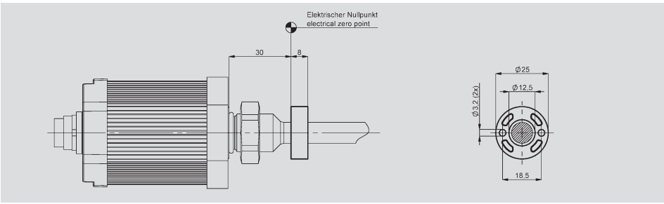
Z-TMI-P02 Ring position marker, Art.No. 005652 weight approx. 10 g
