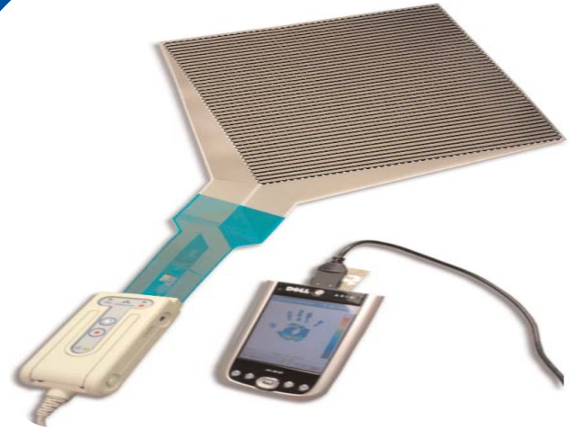
I-Scan Handheld System
