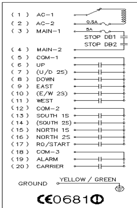
F21-6D/6S Wire Diagram
